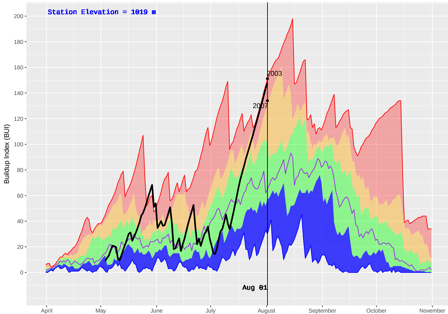
POWDER CREEK (380) : Historical (2001–2016) and Current (2018) Daily Buildup Index (BUI)
