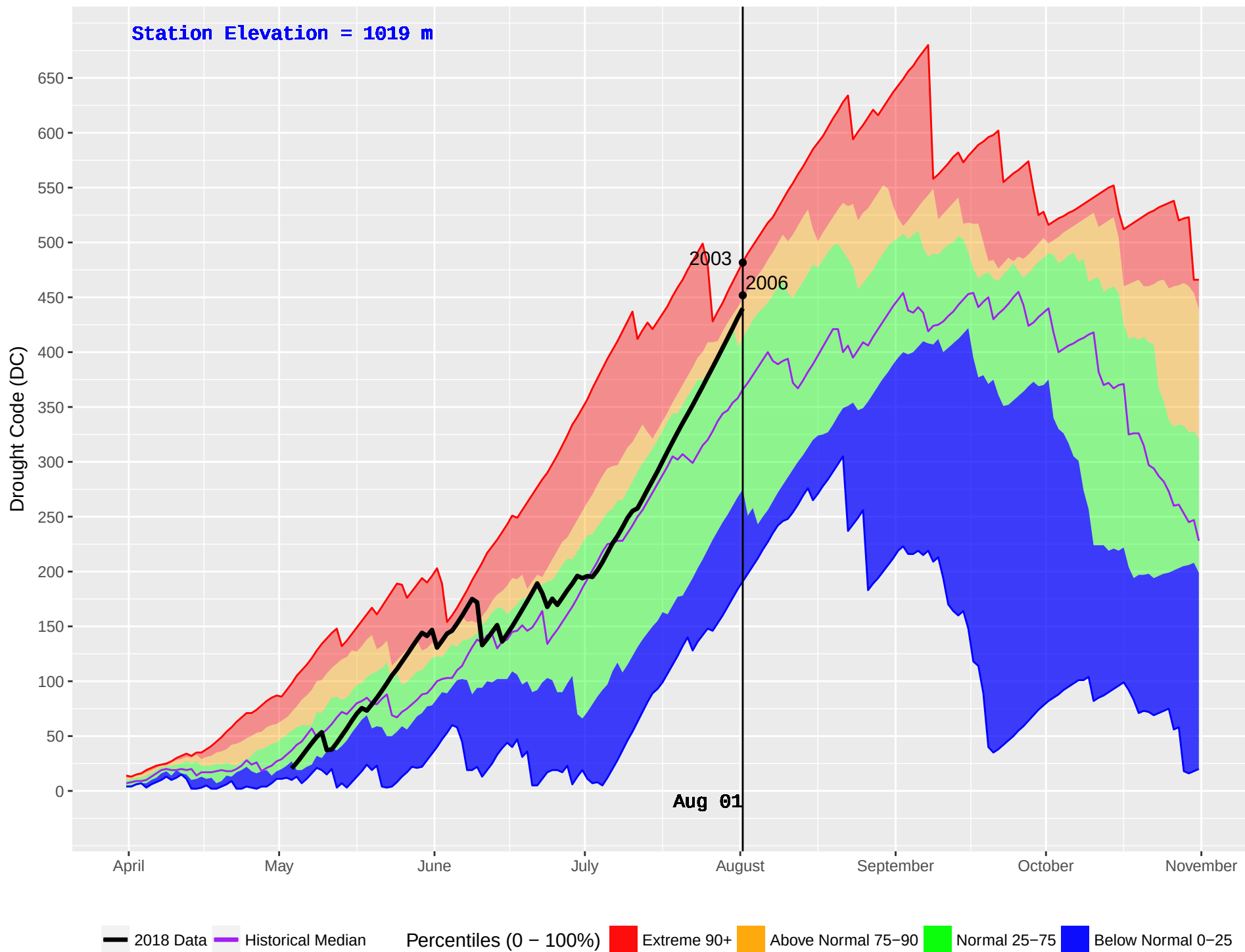
POWDER CREEK (380) : Historical (2001–2016) and Current (2018) Daily Drought Code (DC)
