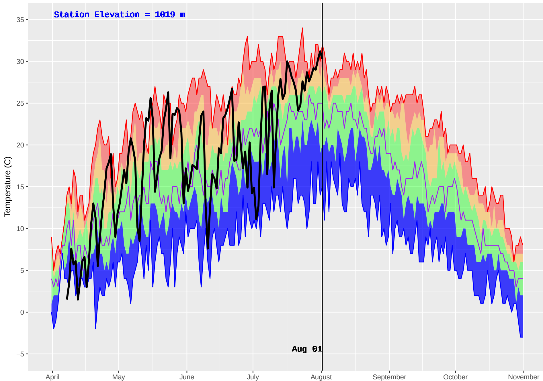
POWDER CREEK (380) : Historical (2001–2016) and Current (2018) Daily Temperature
